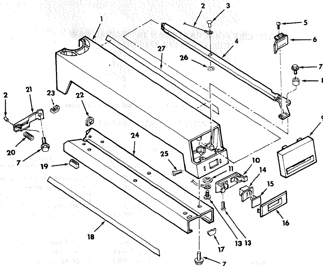
FIGURE 5 - ARM ASSEMBLY
