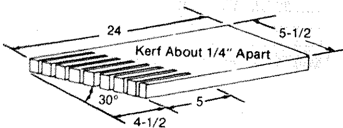
Fig. 116 Featherboard Dimensions
