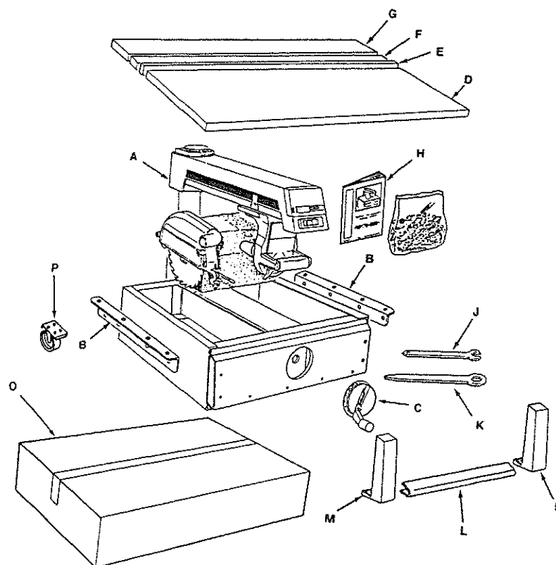
Fig. 10 - Parts for Model 113.278541C
