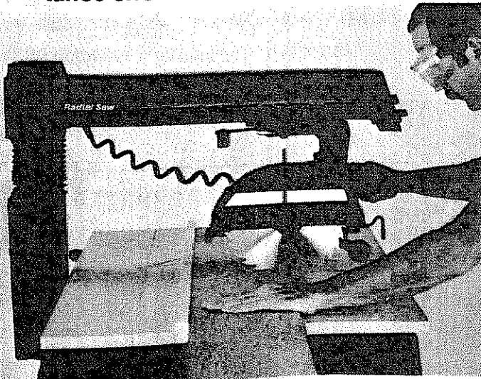
Fig. 86 Blade Distance to Complete Crosscut
