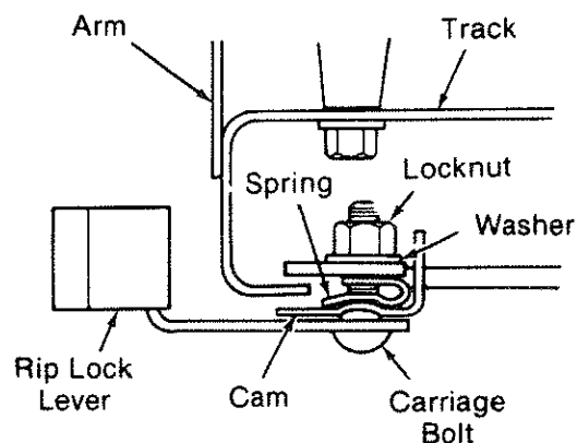
Fig. 130 - Location of Hex Lock Nut
