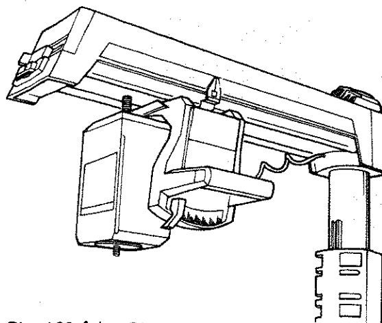
Fig. 108 Arbor Shaft Position When Using Accessory Shaft
