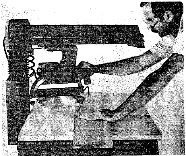
Fig. 84 Compound Crosscut
