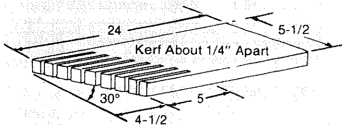
Fig. 116 Featherboard Dimensions
