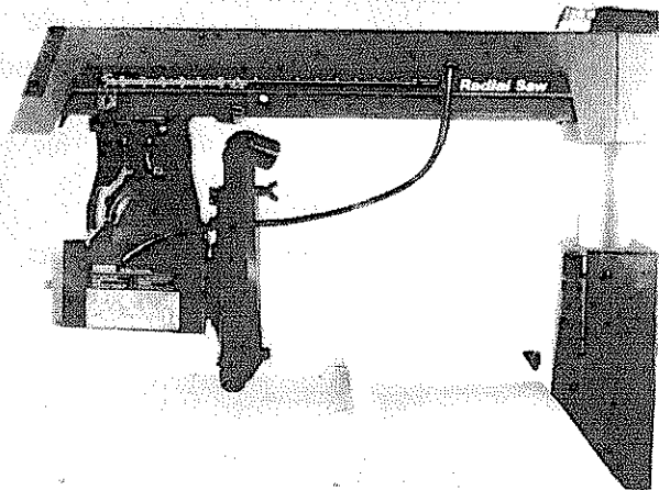
Fig. 102 In-Rip Saw Position
