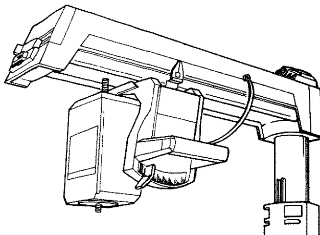
Fig. 108 Arbor Shaft Position When Using Accessory Shaft
