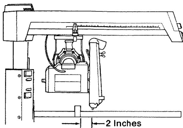
Fig. 78- Out-Rip Saw Position (Infeed End)
