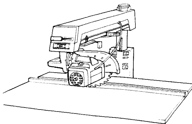
Fig. 75 - In-rip Position
