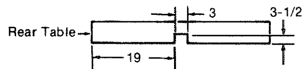
Fig. 115 Rear Table Opening Dimensions
