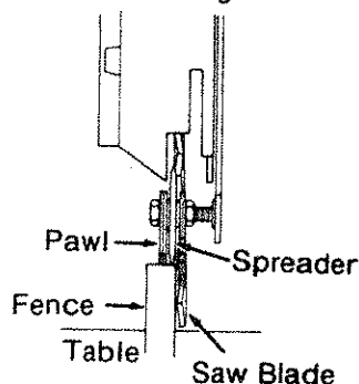
C - Wrong
