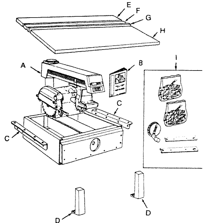
Fig. 10 - Parts for Model 113.278640C
