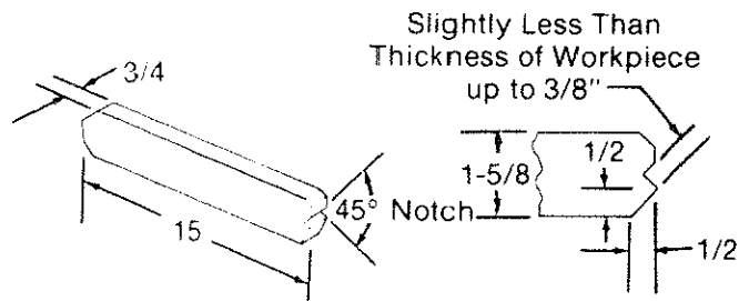
Fig. 109 Push Stick Dimensions
