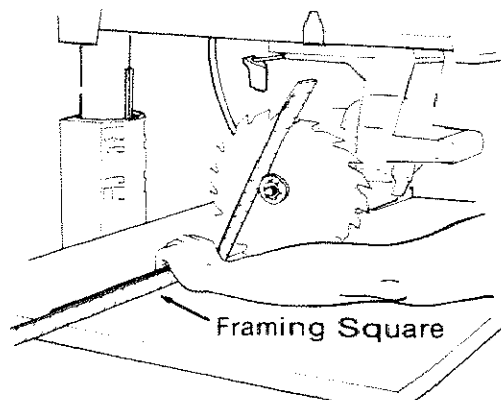
Fig. 60-A - Squaring Blade to Fence
