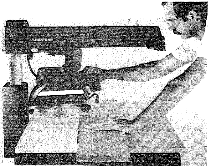
Fig. 84 - Compound Crosscut
