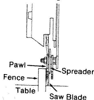
B - Wrong
