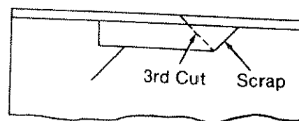
Fig. 119 - Making a 4-Sided Frame
