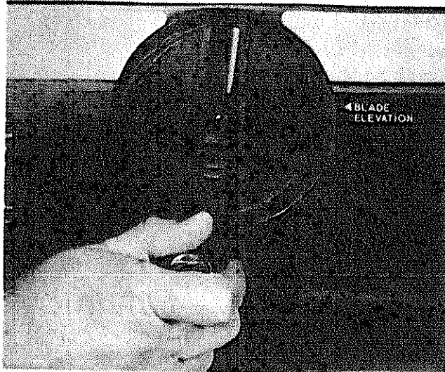
Fig. 34 - Handwheel
