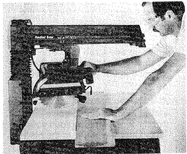
Fig. 84 - Compound Crosscut
