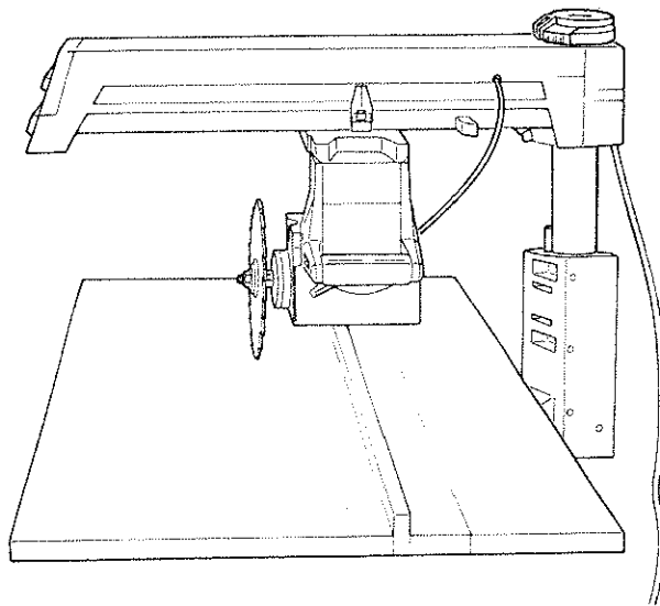
Fig. 63 - Out-rip Position
