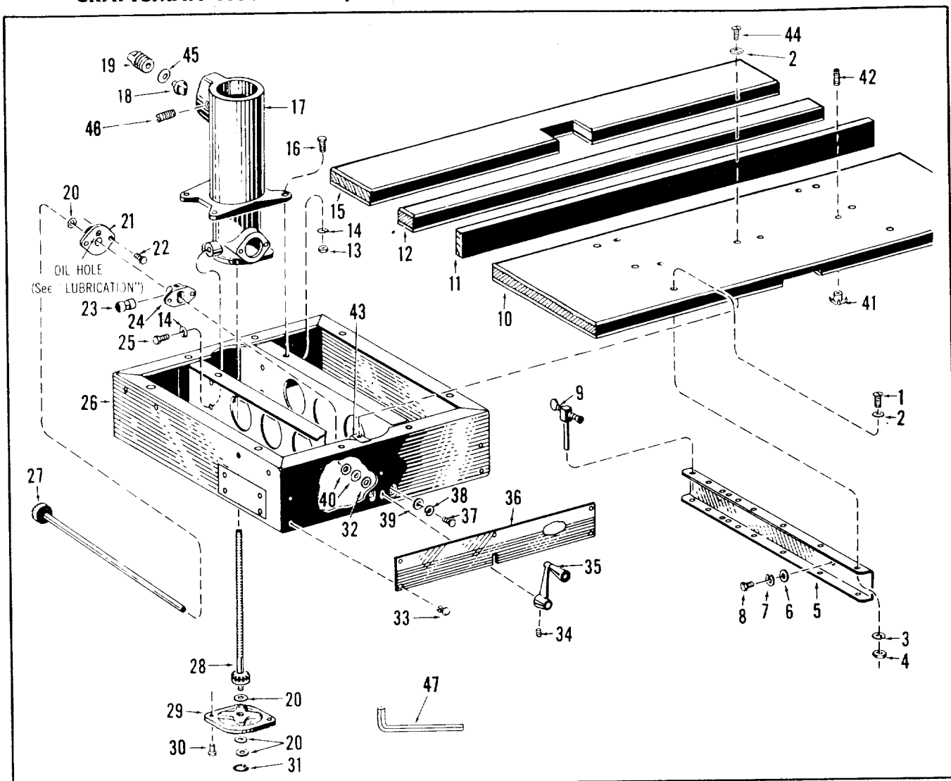
FIGURE 2 PARTS LIST
