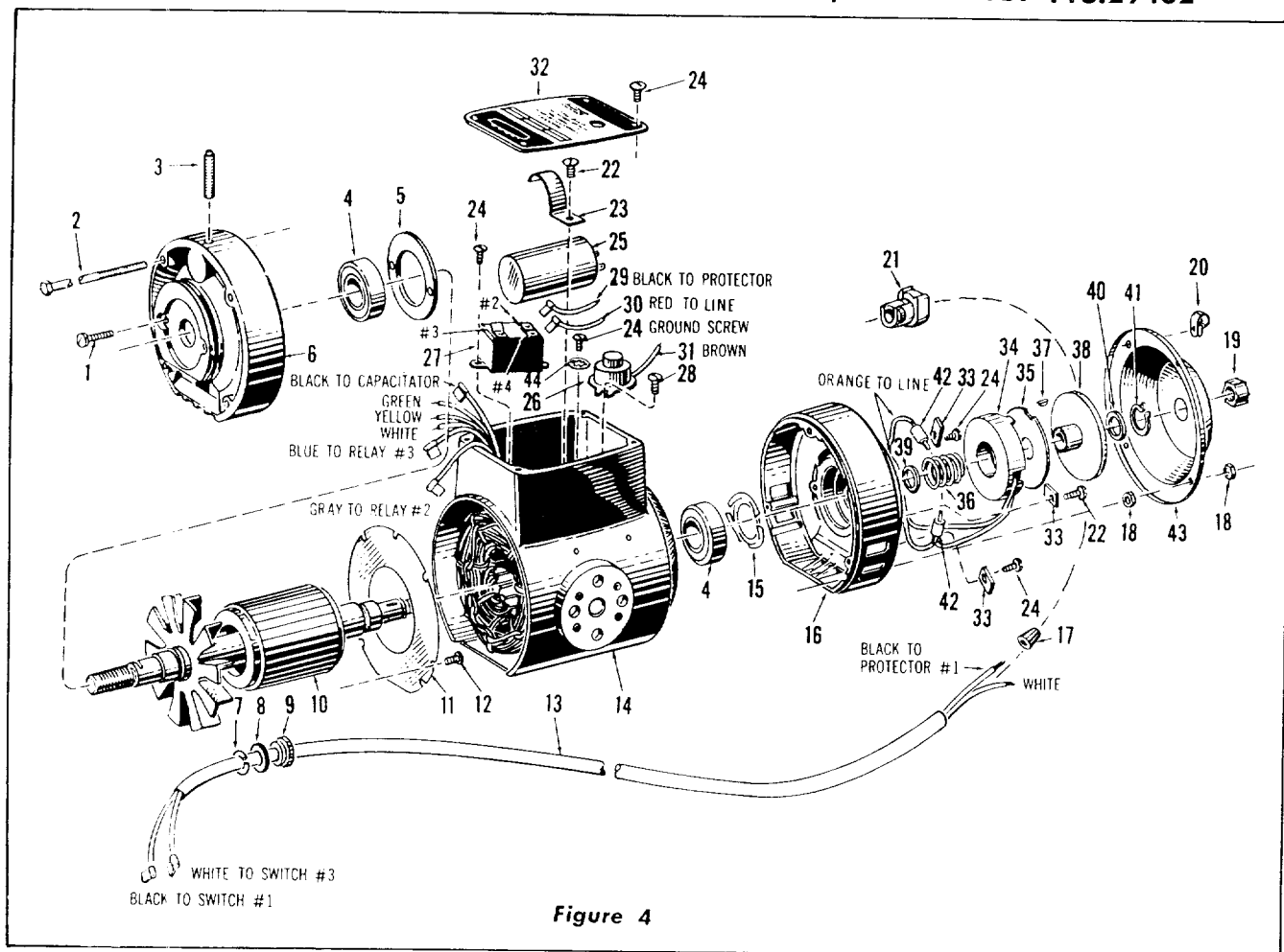
FIGURE 4 PARTS LIST
