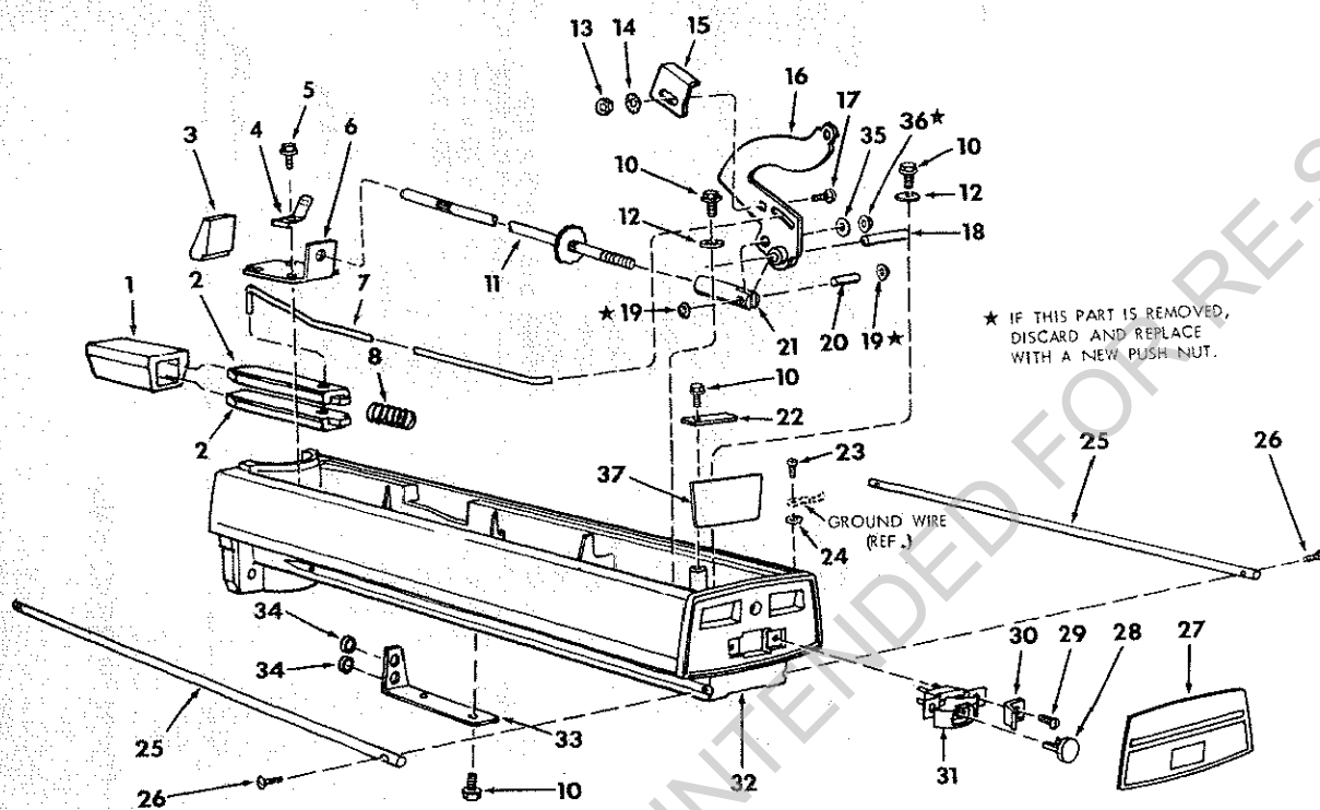
FIGURE 5 – ARM ASSEMBLY
