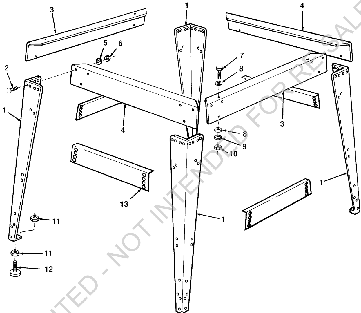
FIGURE 6 - LEG SET
