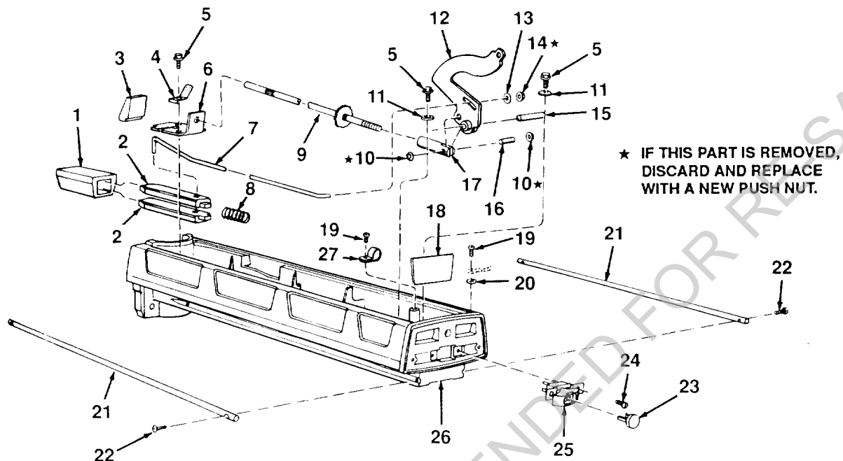
FIGURE 5 – ARM ASSEMBLY
