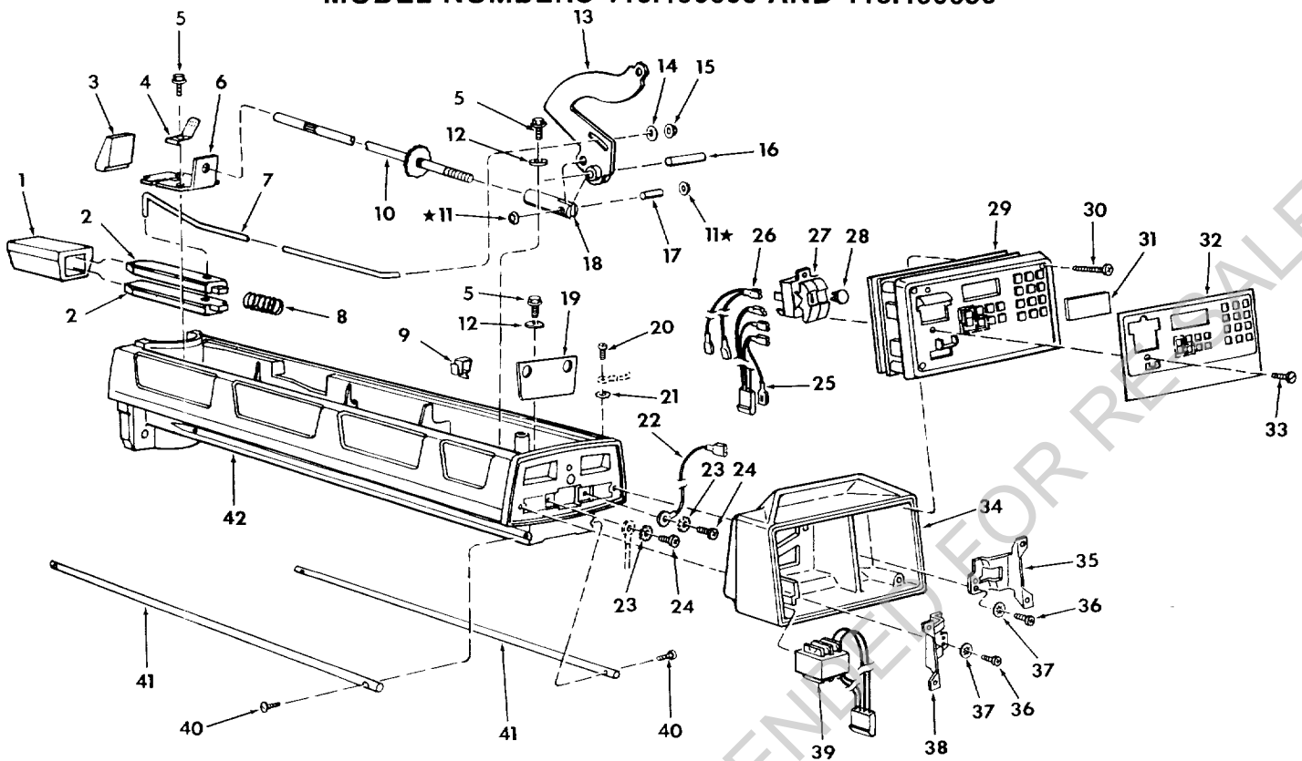
FIGURE 4 - ARM ASSEMBLY
