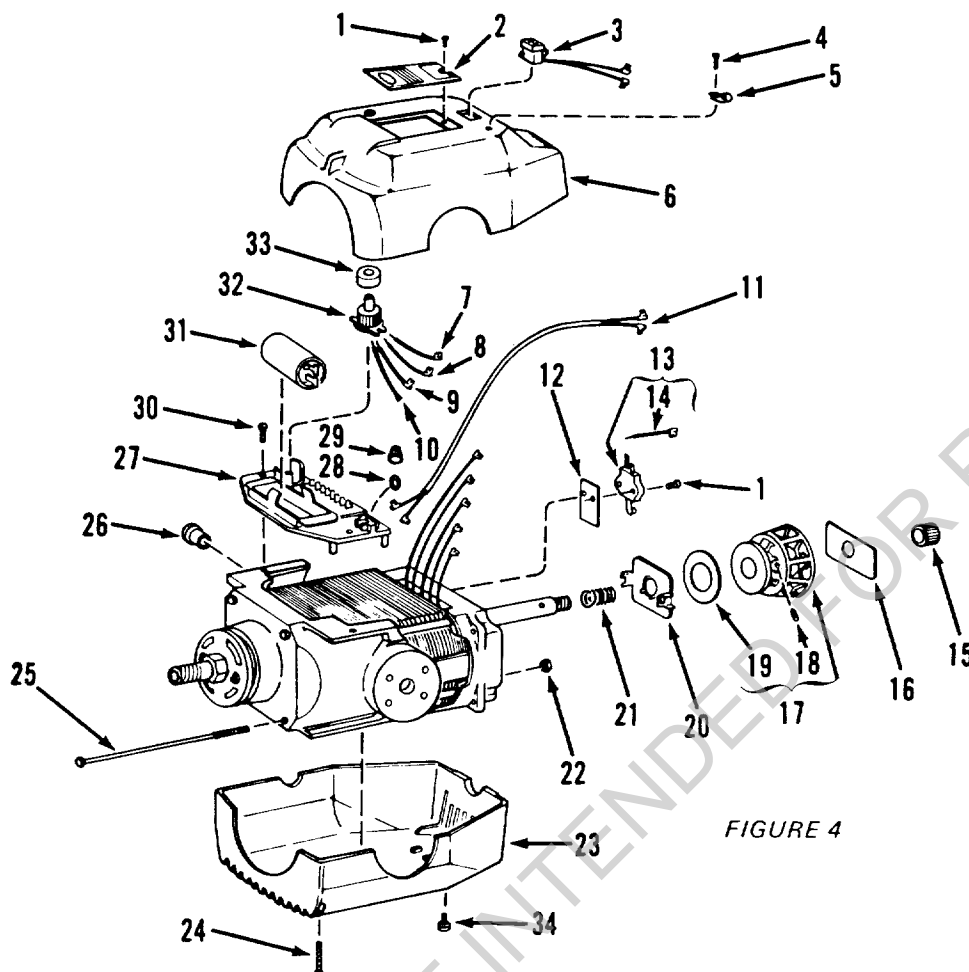
FIGURE 4 PARTS LIST
