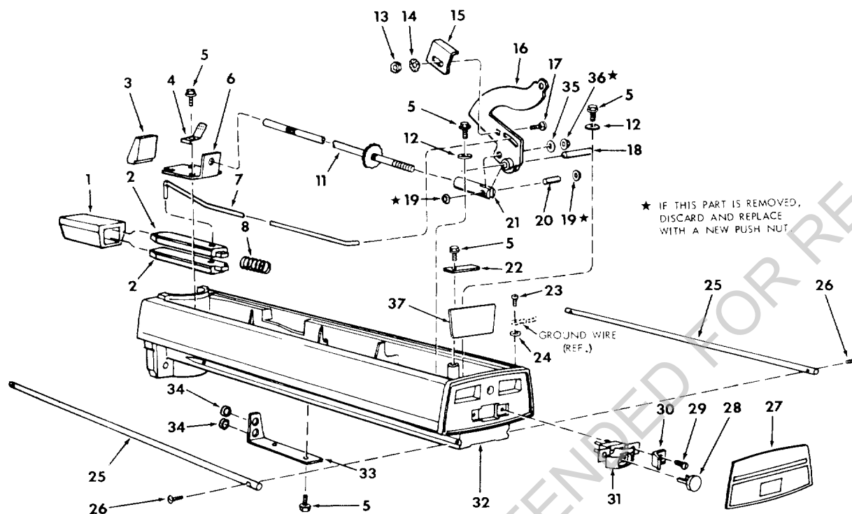
FIGURE 5 – ARM ASSEMBLY
