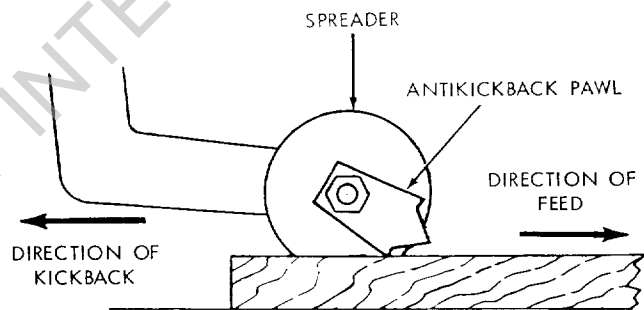
ANTICKICKBACK PAWL POSITION
