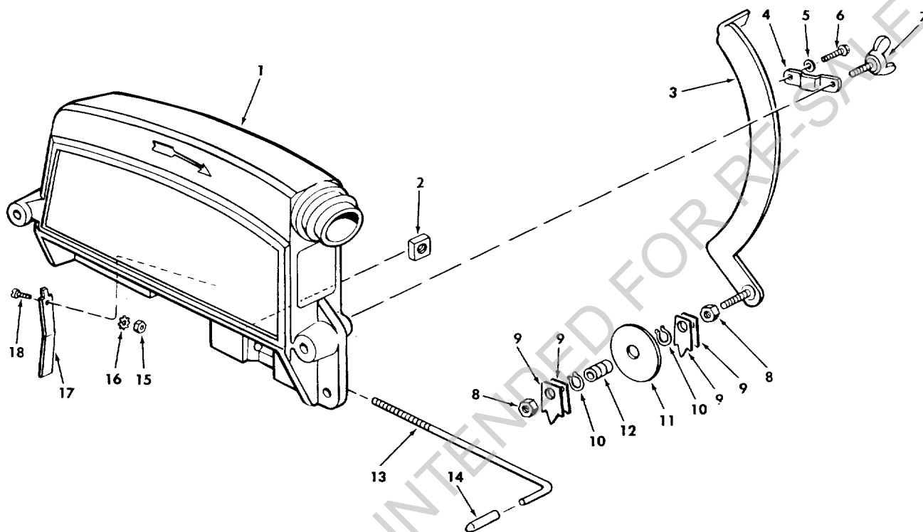
FIGURE 5 – GUARD ASSEMBLY
