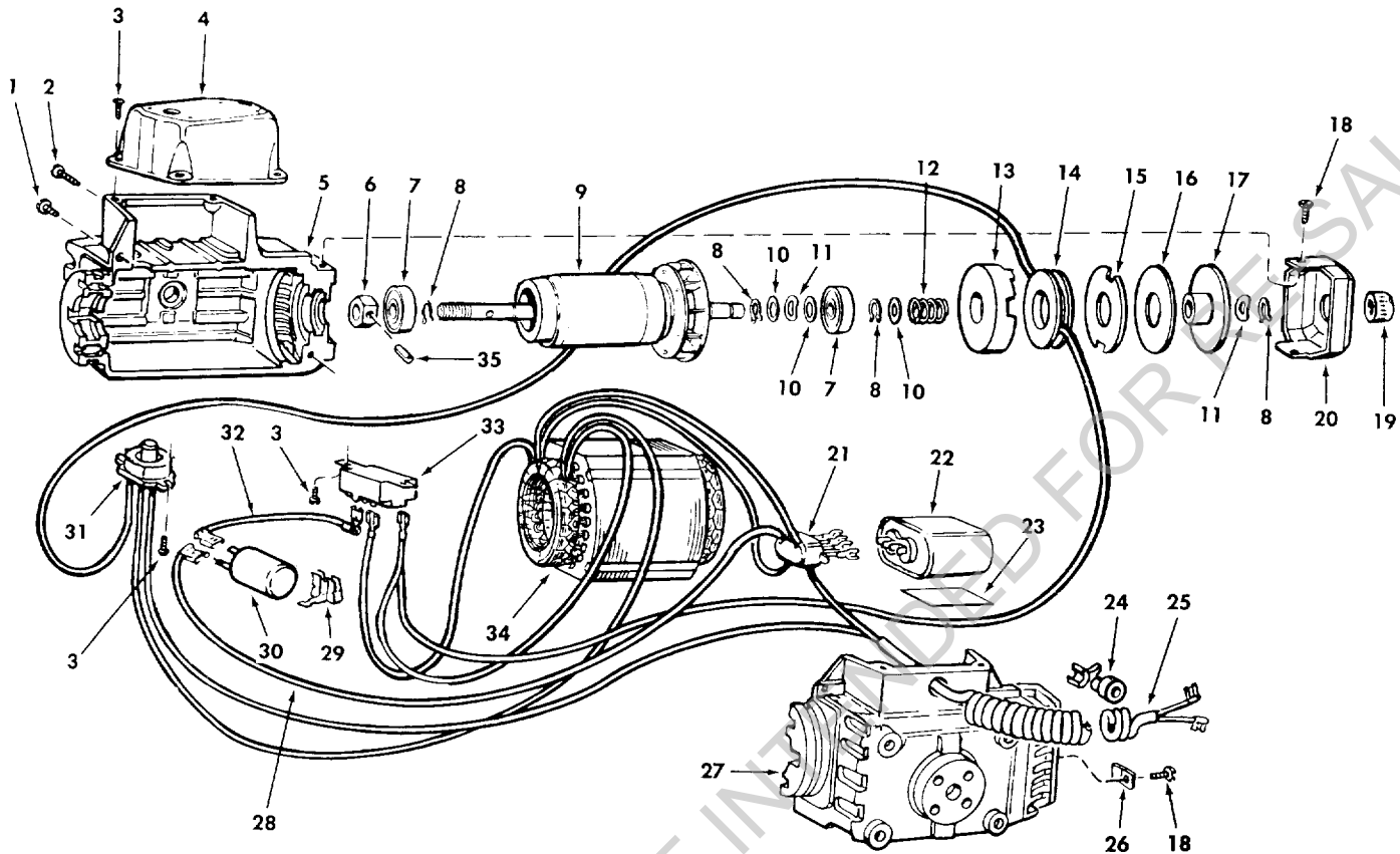
FIGURE 6 — MOTOR ASSEMBLY
