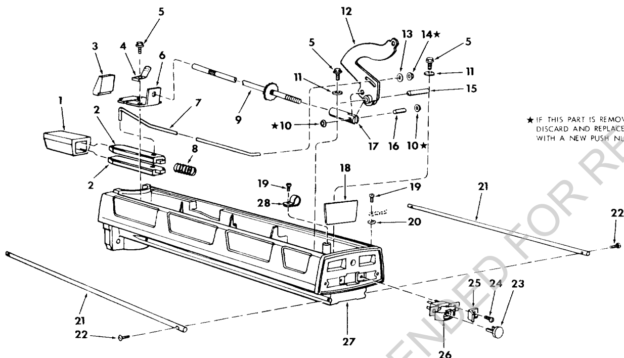
FIGURE 4 – ARM ASSEMBLY
