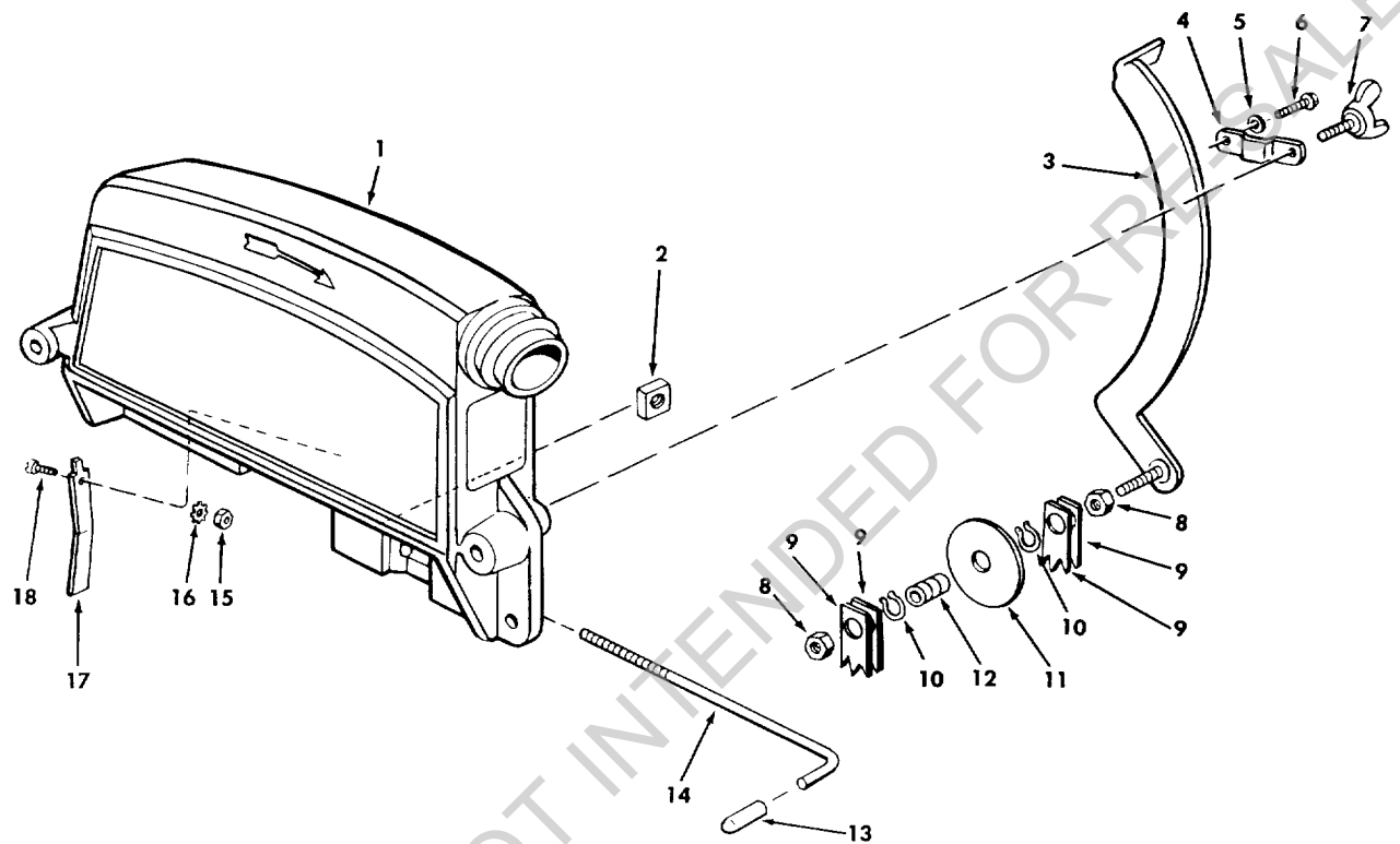
FIGURE 4 — GUARD ASSEMBLY
