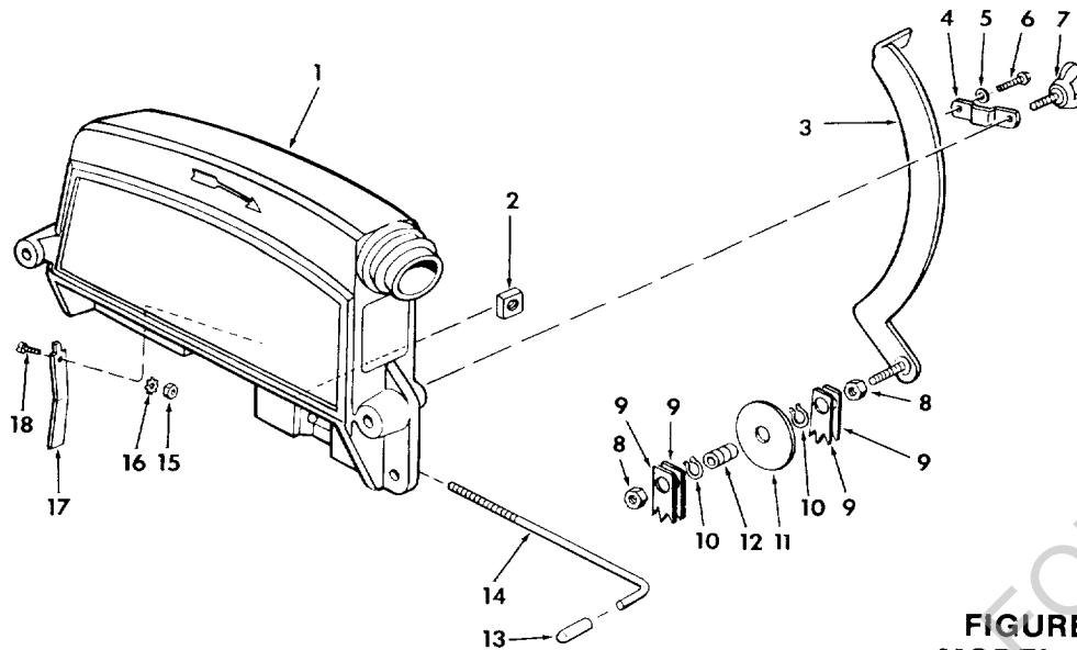
FIGURE 4 — GUARD ASSEMBLY
