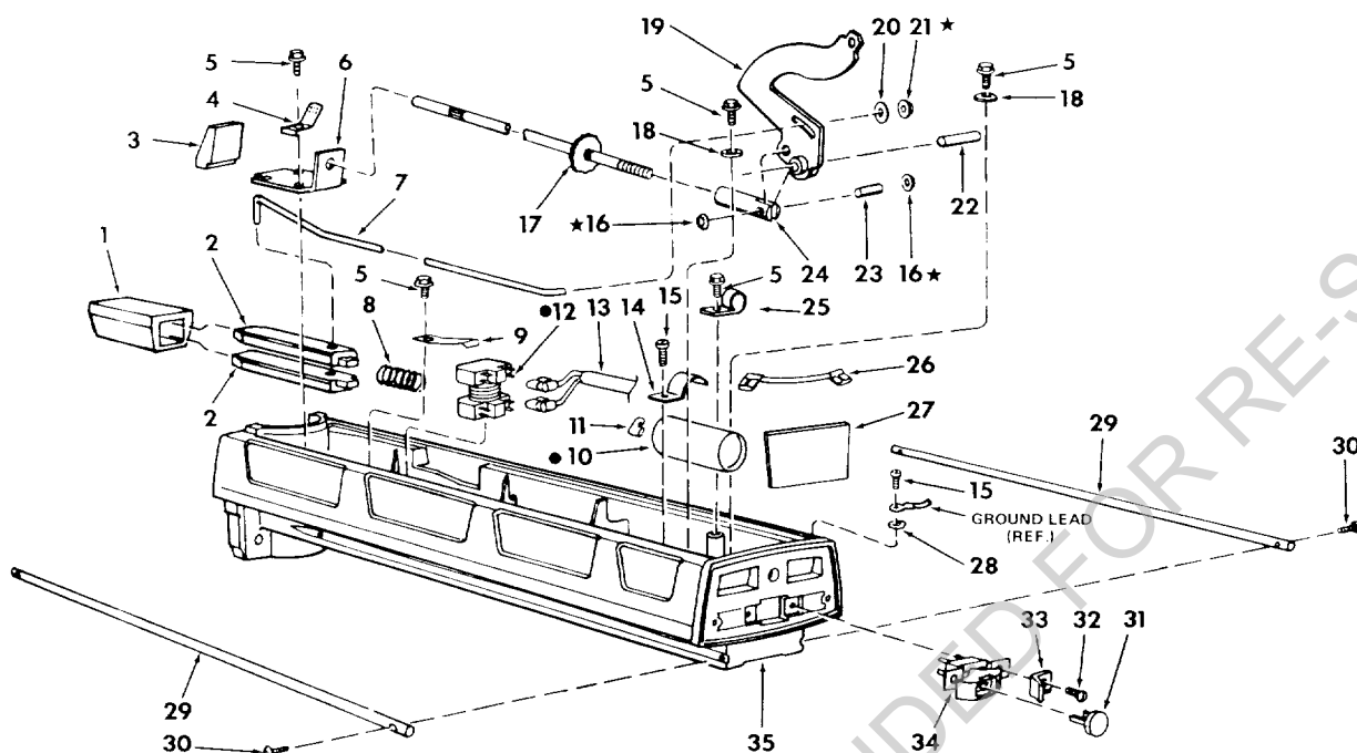
FIGURE 5 — ARM ASSEMBLY
