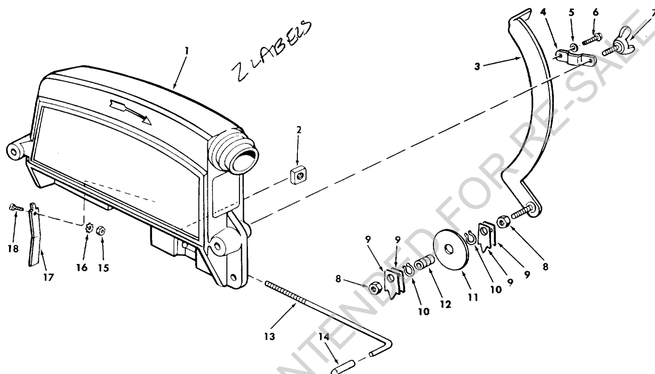
FIGURE 6 — GUARD ASSEMBLY
